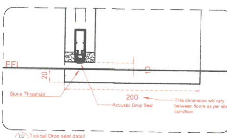
D2 Typical Drop seal detail
